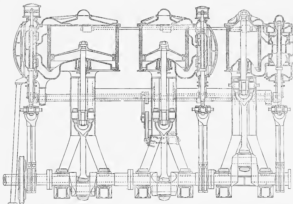
LONGITUDINAL SECTION THROUGH SET OF TRIPLE-EXPANSION ENGINES.
